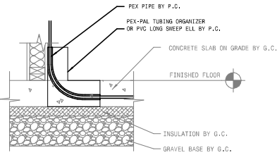
Pipe Penetration Detail NOT TO SCALE
