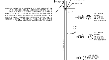
Natural Gas Piping Diagram NOT TO SCALE
