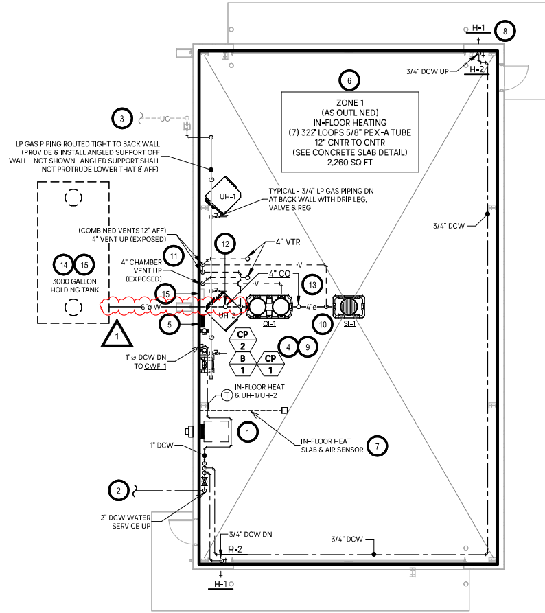
PLUMBING & HYDRONICS PLAN 1/8" = 1'-0" @ 22 X 34 1/16" = 1'-0" @ 11 X 17
