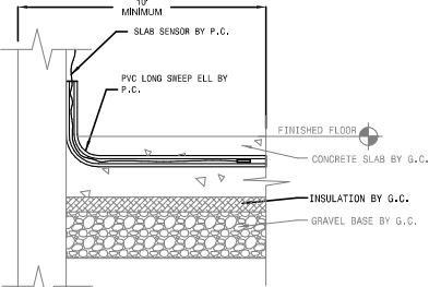
Slab Stat Detail NOT TO SCALE
