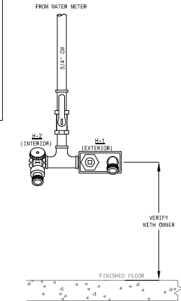
By Alternate - Hydrant Piping Detail NOT TO SCALE
